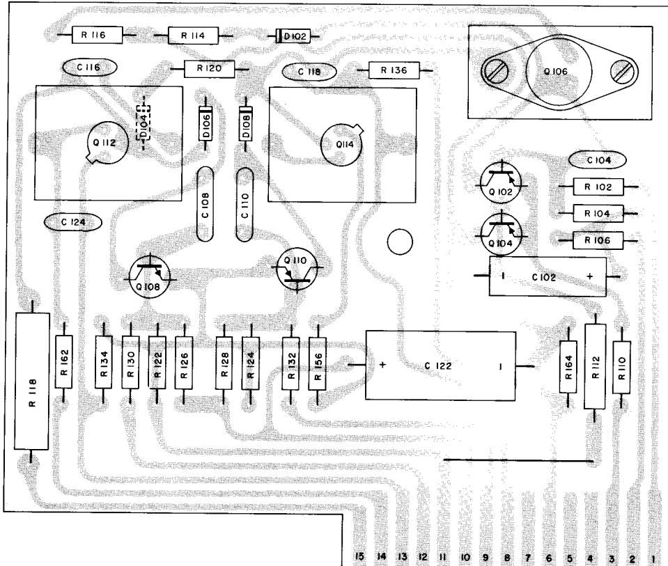
RIGHT CHANNEL POWER OUTPUT PRINTED CIRCUIT BOARD 044-243
