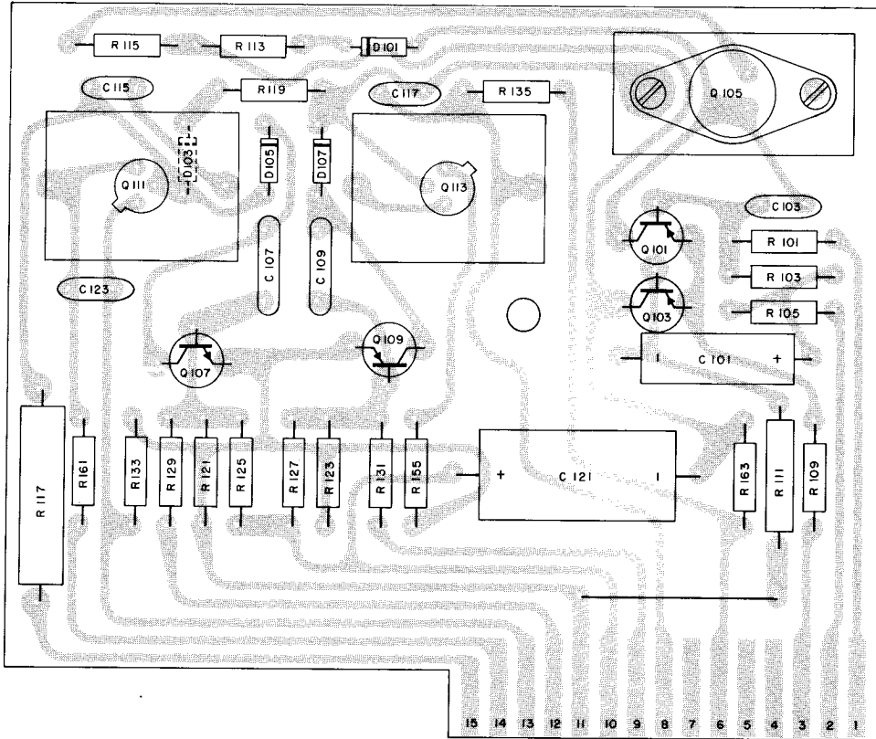
LEFT CHANNEL POWER OUTPUT PRINTED CIRCUIT BOARD 044-243
